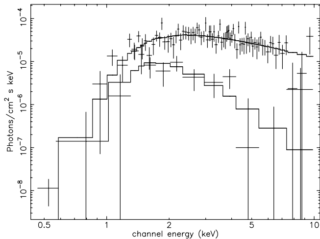
FIG. 3.—Unfolded spectra of [N03] 75 in the two XMM-Newton observations, shown along with the best-fit power law (see Table 2). The upper spectrum presents the EPIC MOS2 data of revolution 0357, and the lower one corresponds to the EPIC MOS1 data of revolution 0157 (in the other cameras, the source was either in a gap, out of the FOV, or close to the edge of the FOV). In revolution 0157, the luminosity in the 0.4–10 keV energy range has decreased by greater than 200%, while the power-law slope has steepened from 1.1 to 3.9.
