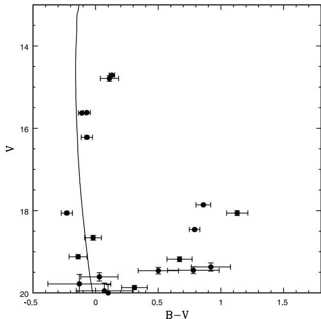
FIG. 2.—Color-magnitude diagram of the counterparts listed in Table 3. The error bars correspond to the dispersion of the measured data. Counterparts with V > 20 mag were not included since their photometry is very uncertain. The solid line shows an isochrone of 5 Myr for Z = 0.004 (Lejeune & Schaerer 2001) transformed using a distance of 59 kpc and reddened with R_V = 3.3 and E(B-V) of 0.14 mag (Massey et al. 1989).
