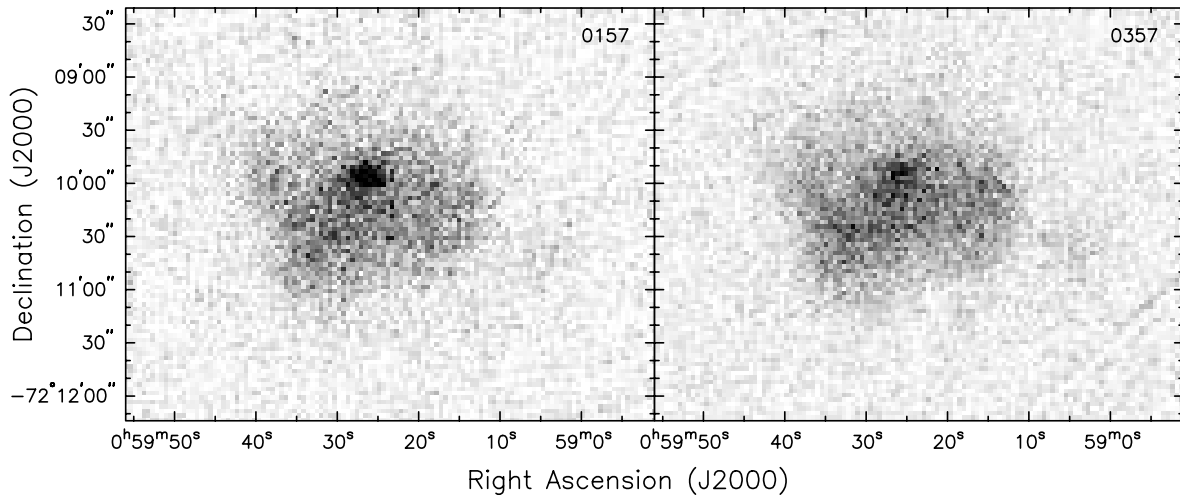
FIG. 4.—EPIC image of the SNR and HD 5980 for both observations. The cluster NGC 346 is just barely visible to the southwest of the SNR, at position 0^{\text{h}}59^{\text{m}}04^{\text{s}} , -72^{\circ}10'35'' (whereas HD 5980 is at 0^{\text{h}}59^{\text{m}}26^{\text{s}} , -72^{\circ}09'53'' ). This figure uses the same event lists as Fig. 1.
