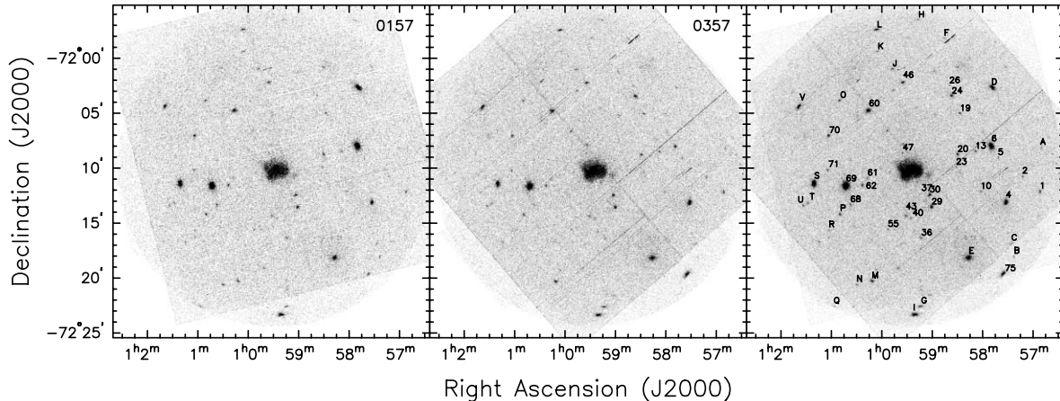
FIG. 1.—NGC 346 field as seen by the EPIC instruments on board XMM-Newton . Left : Data from revolution 0157. Middle : Data from revolution 0357. Right : Combined data from both revolutions with identification numbers (see Table 1 for a precise list of positions). Note that these figures were made by keeping the EPIC pn events with a pattern between 0 and 12 and passing through the #XMMEA_EP filter.
