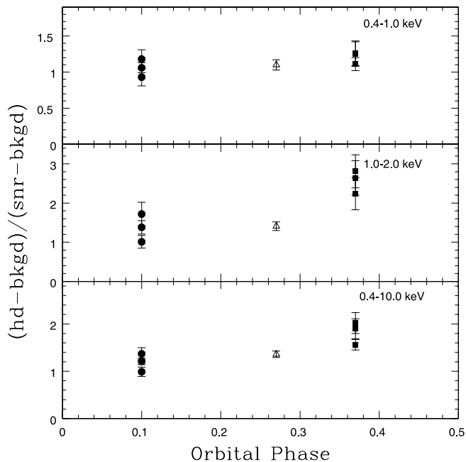
FIG. 5.—Evolution of the diagnostic ratio for HD 5980 (see text): open triangles show the Chandra data, filled squares the XMM-Newton data from revolution 0157, and filled circles the XMM-Newton data from revolution 0357. The three symbols for each XMM-Newton observation correspond to the ratio evaluated for the three EPIC cameras. The hard X-ray luminosity of HD 5980 is clearly increasing in the XMM-Newton observation from revolution 0157.
